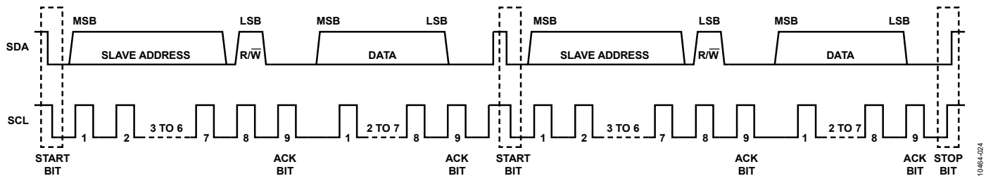
Figure 25. I²C Repeated Start Sequence
