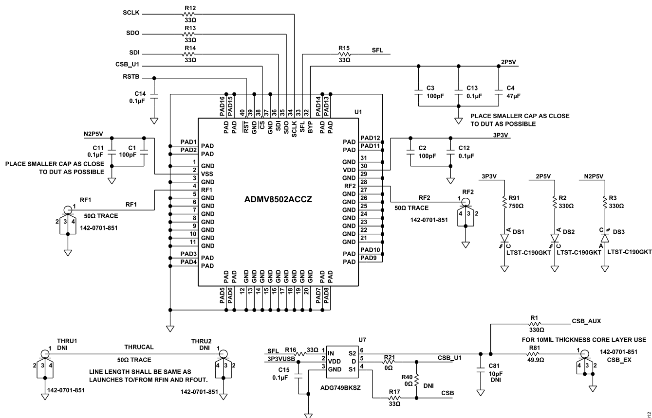
Figure 12. ADMV8502-EVALZ Schematic, Page 1
