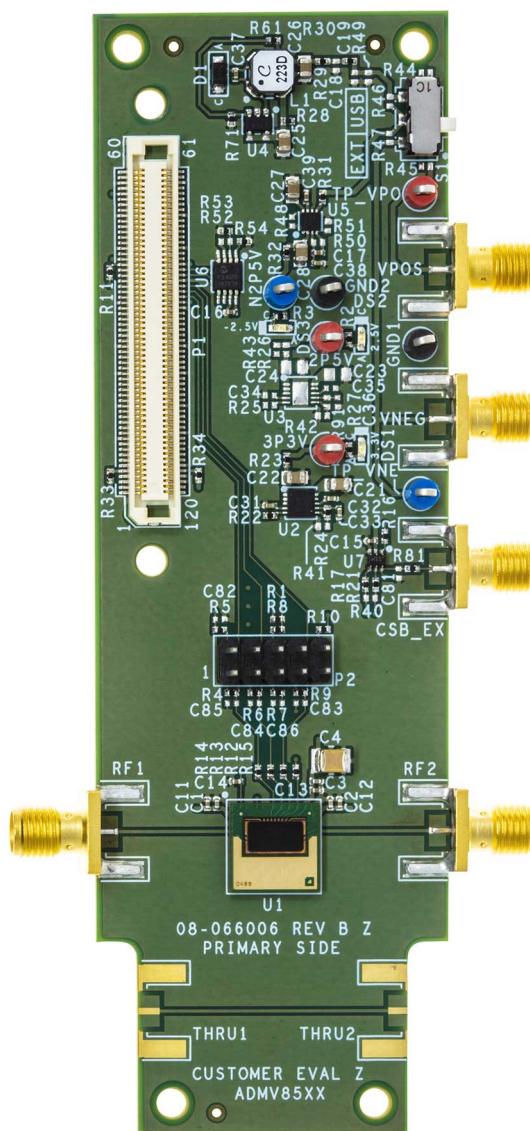
Figure 1. ADMV8502-EVALZ Evaluation Board Photograph
