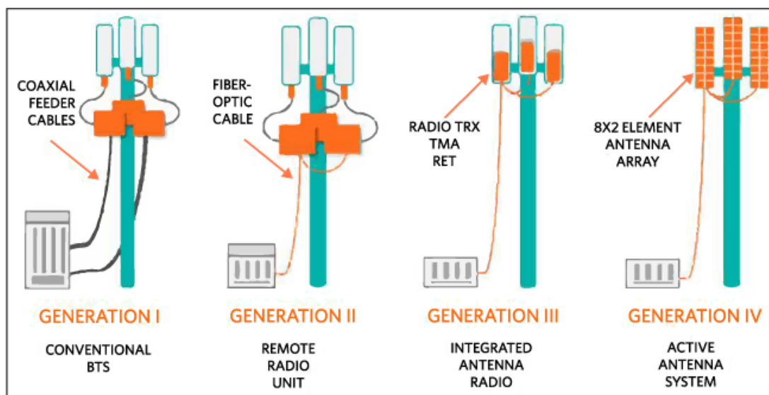
Figure 7. The evolution of base stations from the first-generation BTS through contemporary Generation IV.
