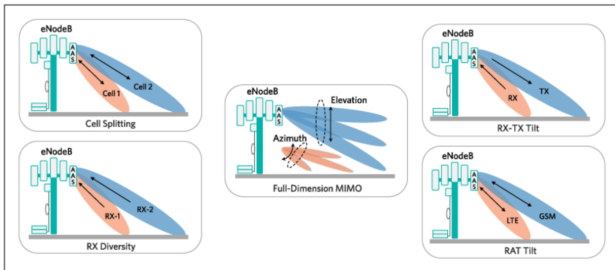
Figure 9. Several AAS beamforming and beam steering applications are possible for macro cell sites.
