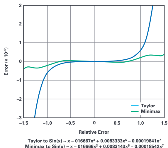
Figure 3. Unlike the Taylor-MacLaurin method defined around 0, the minimax sine approximation approach minimizes and equalizes the maximum relative error over the [-\pi/2 to +\pi/2] interval.
