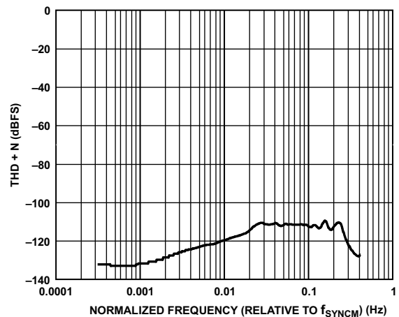
Figure 18. PDM Total Harmonic Distortion + Noise (THD + N) vs. Normalized Frequency (Relative to f_{\text{SYNCM}} ), f_{\text{SYNCM}} = 48 \text{ kHz}
