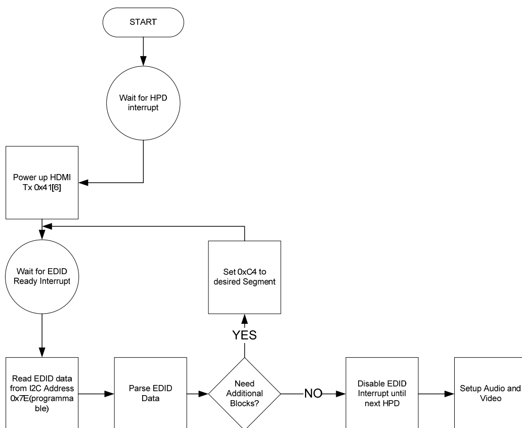
Figure 23 Reading EDID through the ADV7511W
