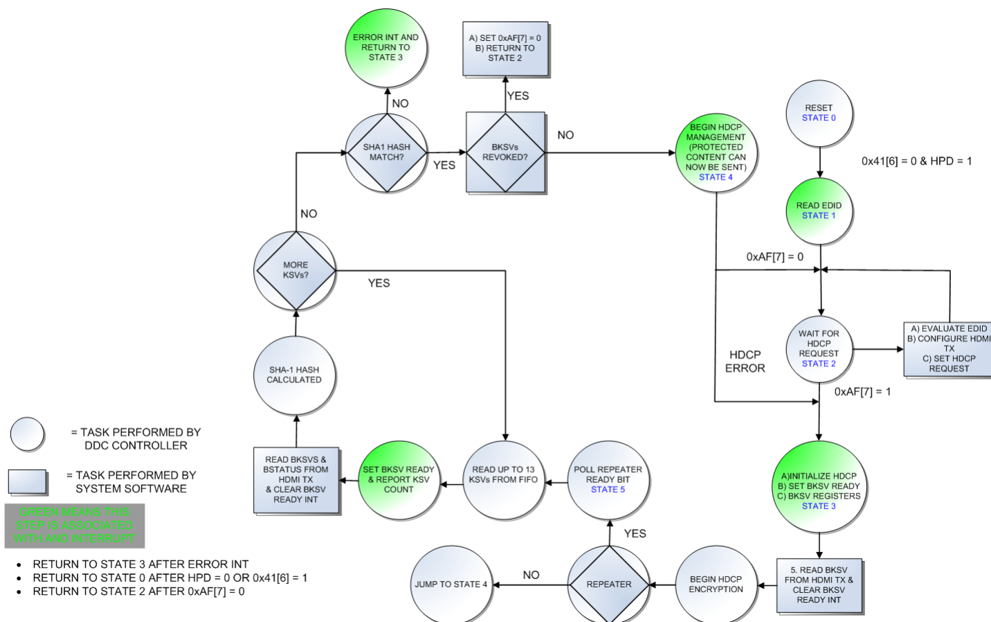
Figure 31 ADV7511W EDID and DDC Controller Functional Flow
