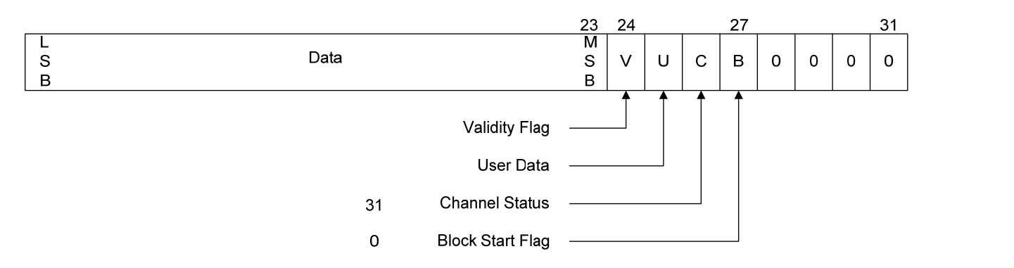
Figure 14 Sub-Frame Format for ADV7511W
