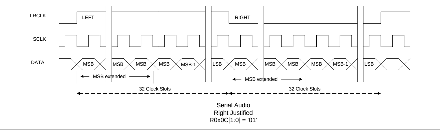
Figure 16 Right-Justified Timing
