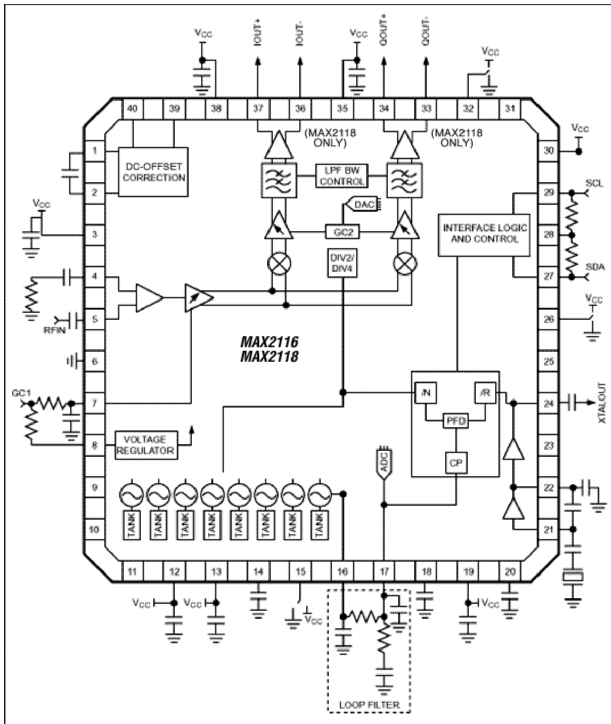
Figure 1. MAX2116/MAX2118 typical operating circuit.
