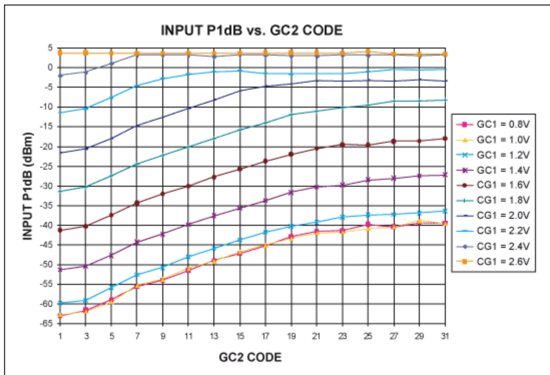
Figure 2. MAX2116 Input P_{1db} vs. GC2 code.
