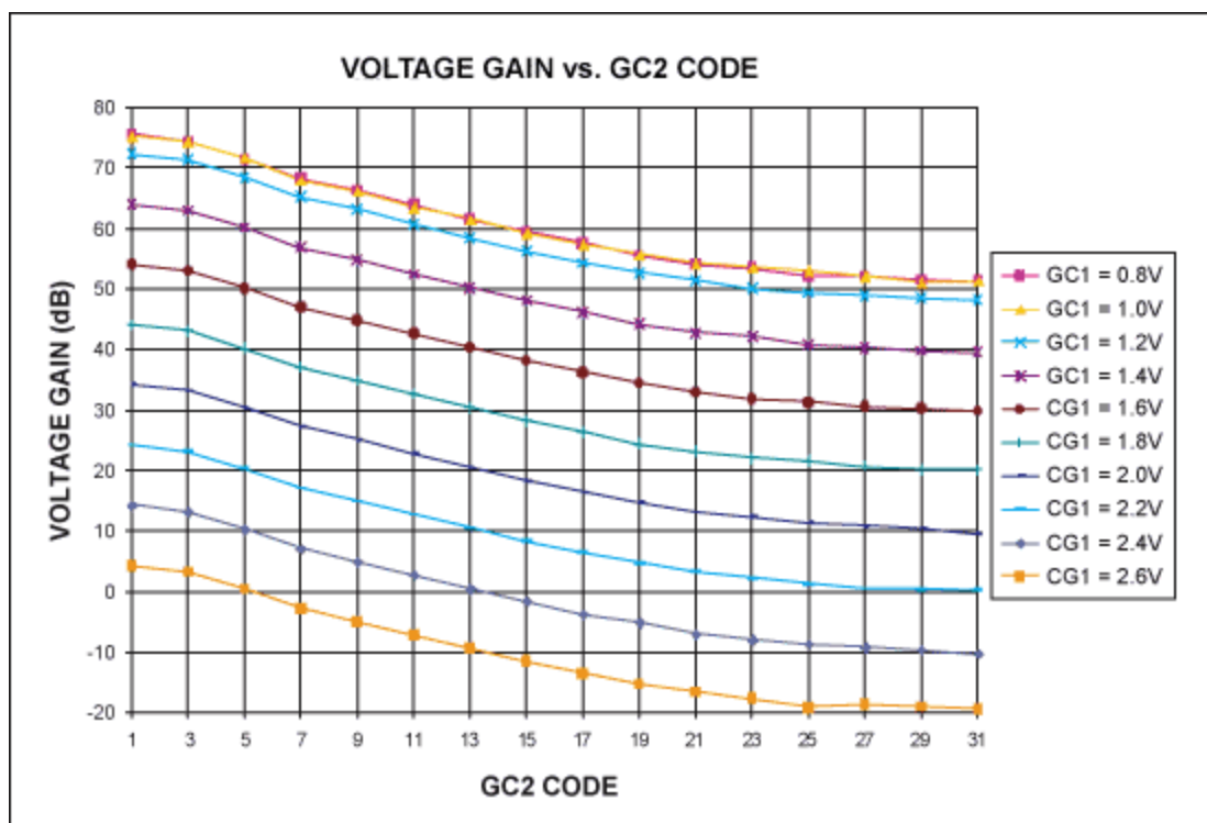
Figure 3. MAX2116 voltage gain vs. GC2 code.
