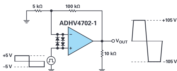
Figure 1. ADVH4702-1 output swing circuit and capability.
