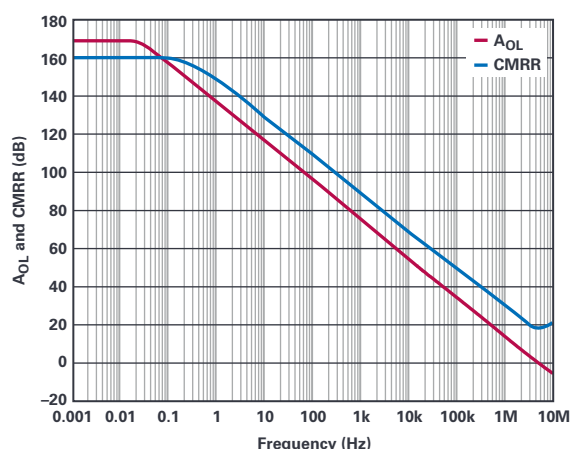
Figure 2. ADVH4702-1 precision performance.
