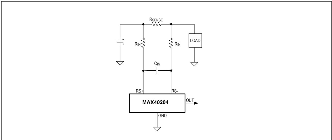
Figure 3. Differential Input Filtering
