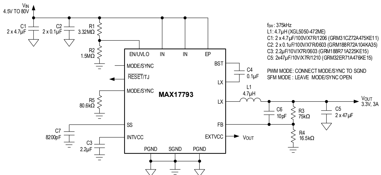
Figure 8. 3.3V Output with 400kHz Switching Frequency
