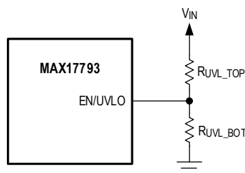
Figure 5. Setting the Input Undervoltage Lockout
