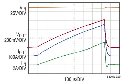
65V IN Short-Circuit Start-Up
