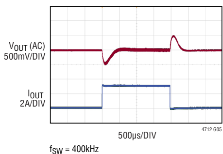
Transient Response, 5V IN to 12V OUT
