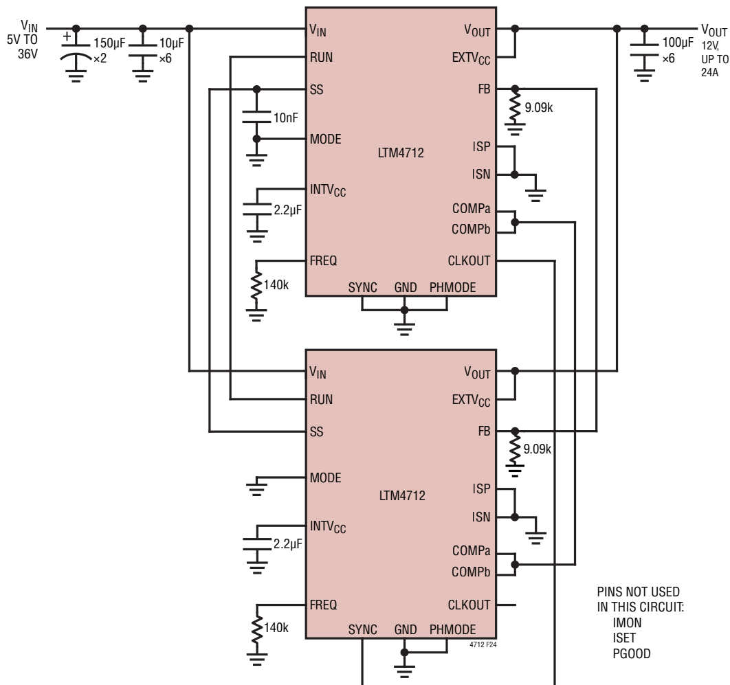
Figure 24. 2 \times LTM4712 Parallel to Provide Up to 24A Output Current
