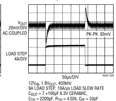
Dual Phase Single Output 25% (9A) Transient Response at 1.8V Output
