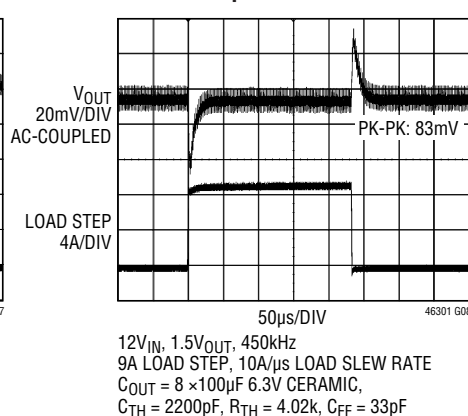
Dual Phase Single Output 25% (9A) Transient Response at 1.5V Output
