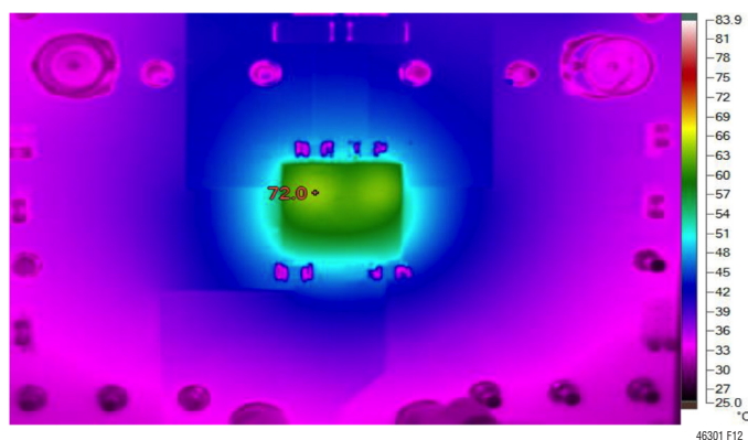
Figure 12. Thermal Image 12V to 1.0V, 36A with 200LFM Airflow without Heat Sink
