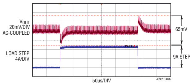
25% Load Step Transient Response, \pm 3\% Output Regulation Window, 12V IN , 1.2V OUT , 36A with 5× 220μF Ceramic Capacitor
