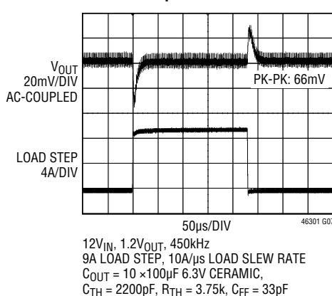
Dual Phase Single Output 25% (9A) Transient Response at 1.2V Output
