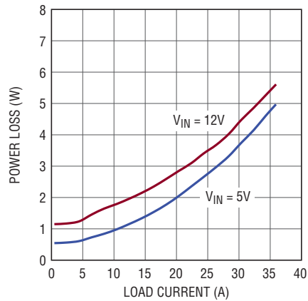
Figure 16. 1.5V Power Loss Curve
