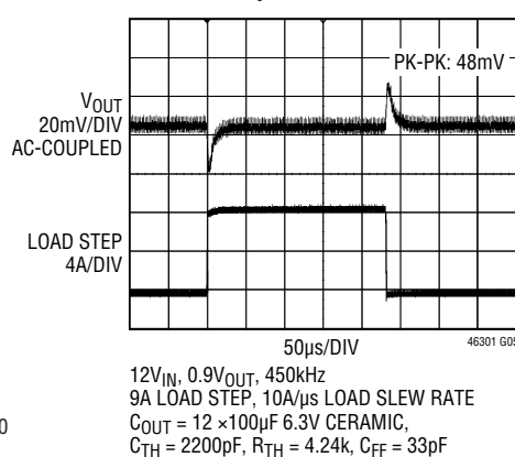
Dual Phase Single Output 25% (9A) Transient Response at 0.9V Output
