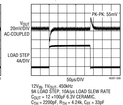
Dual Phase Single Output 25% (9A) Transient Response at 1V Output
