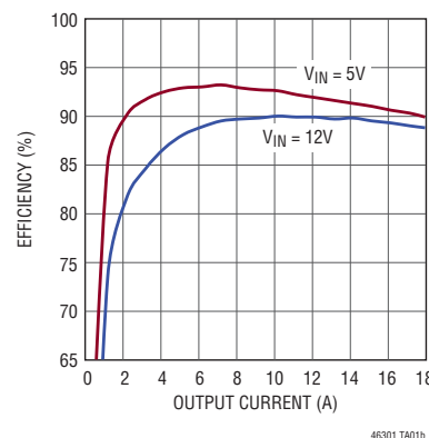
1.2V Output Efficiency vs I OUT
