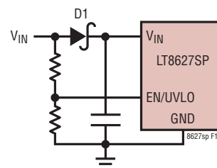
Figure 12. Reverse V IN Protection
