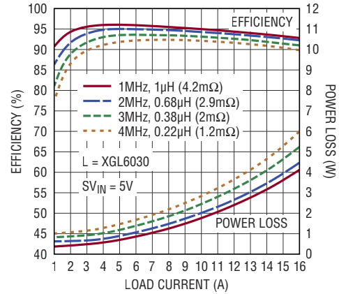
12V IN to 3.3V OUT Efficiency
