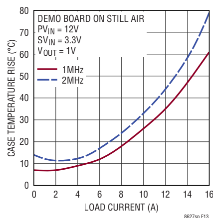
Figure 13. Case Temperature Rise
