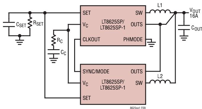
Figure 9. Paralleling Two LT8625SP/LT8625SP-1 Devices
