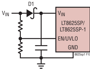
Figure 10. Reverse V_{IN} Protection
