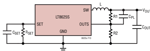
Figure 13. Configuring the LT8625S for Output Voltages Above 6V
