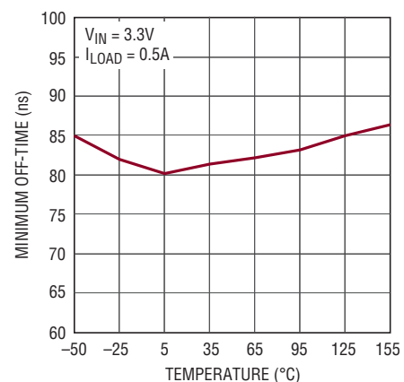
Minimum Off-Time
