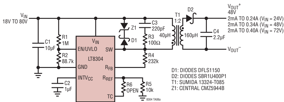
18V to 80V IN /48V OUT Isolated Flyback Converter
