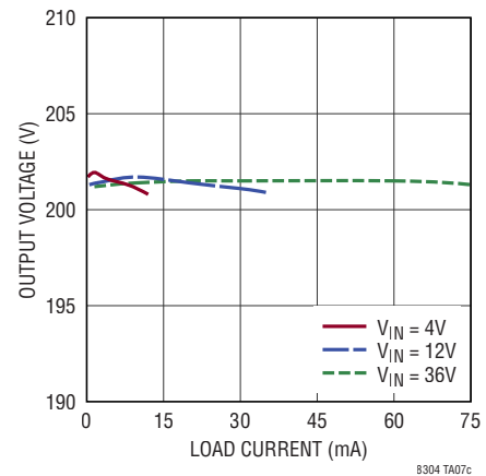
Load Regulation, V_{OUT} = 200V
