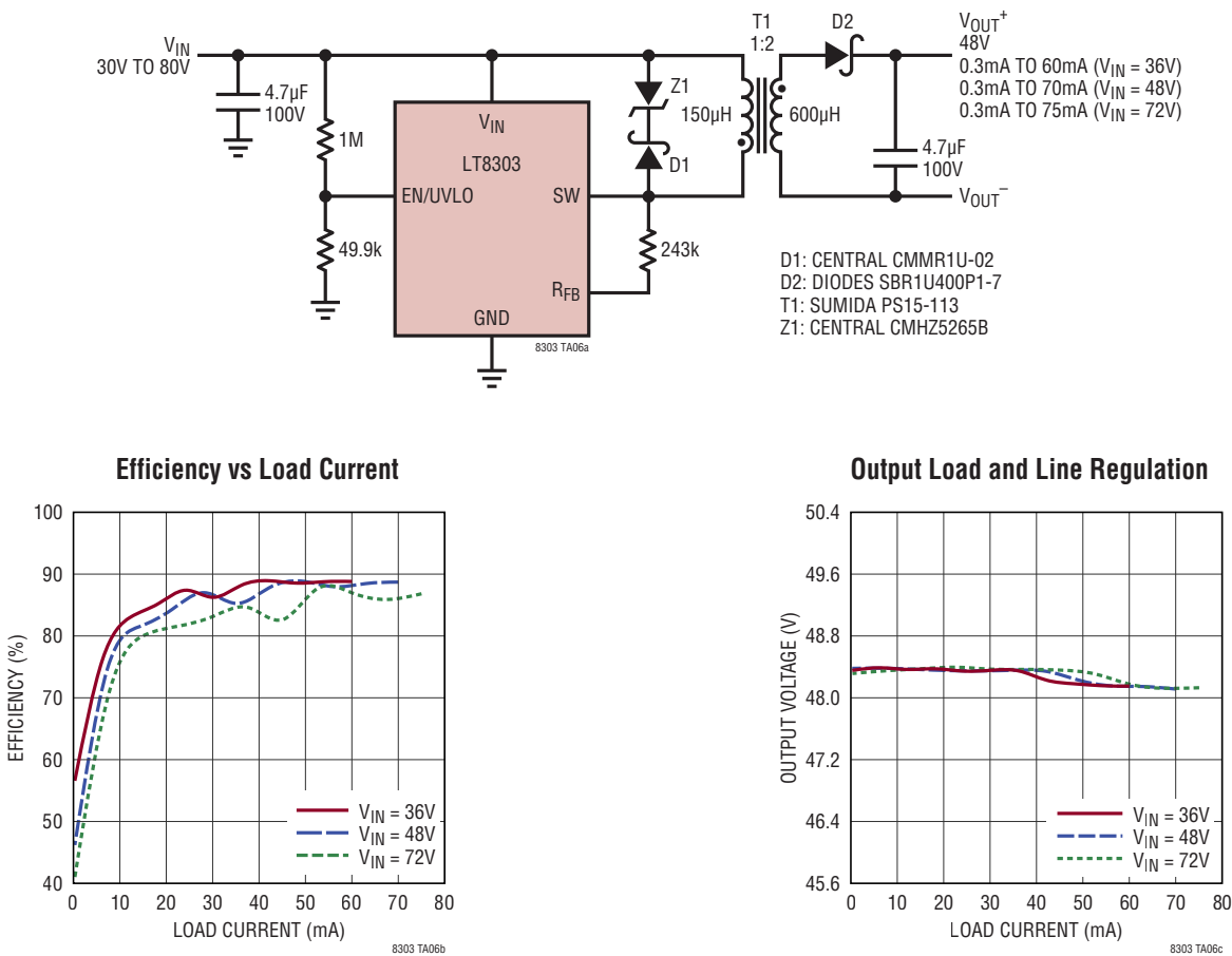
30V to 80V IN , 48V OUT Isolated Flyback Converter
