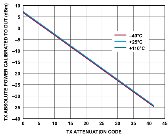
Figure 254. Transmitter Absolute Power Calibrated to DUT vs. Transmitter Attenuation Code, Baseband Frequency = 2.1 kHz, Backoff = 0.2 dBFS
