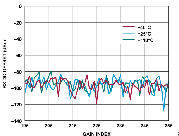
Figure 24. Receiver DC Offset vs. Gain Index, Baseband Frequency = 5.6 MHz, ADC = High Performance
