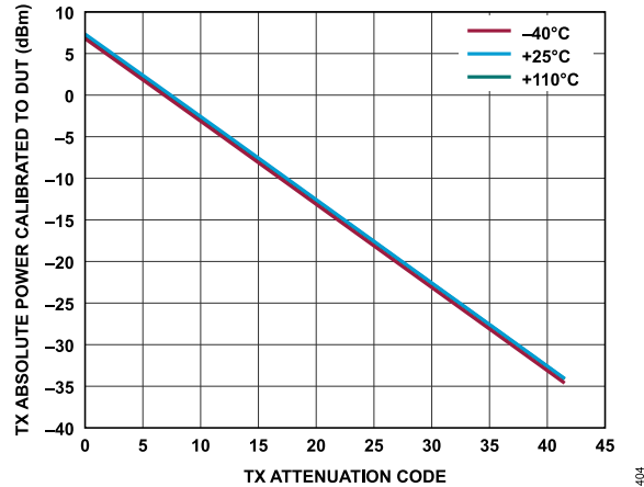
Figure 273. Transmitter Absolute Power Calibrated to DUT vs. Transmitter Attenuation Code, Baseband Frequency = 2.1 kHz, Backoff = 0.2 dBFS
