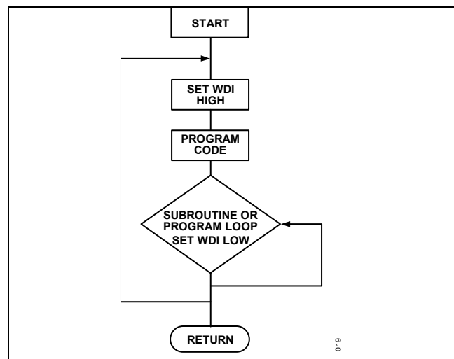
Figure 16. Watchdog Flow Diagram
