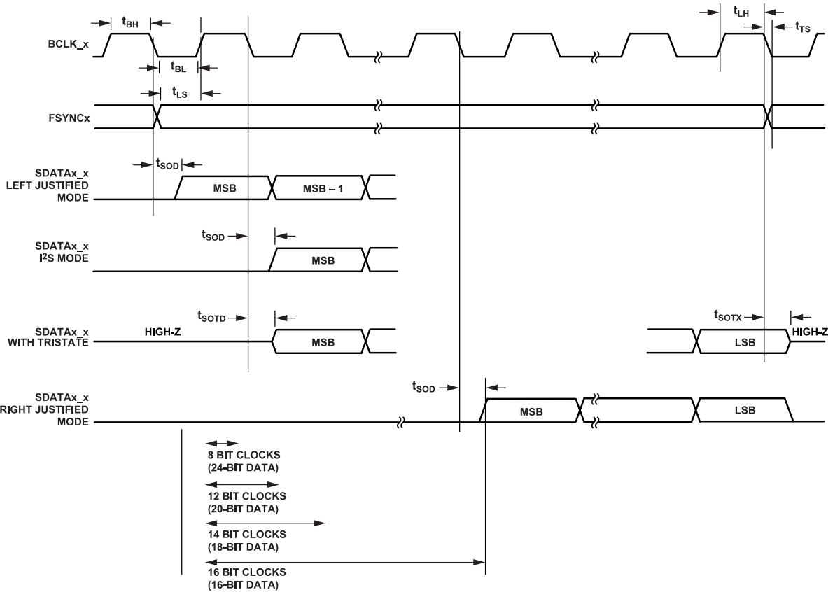
Figure 3. Serial Output Port Timing Diagram
