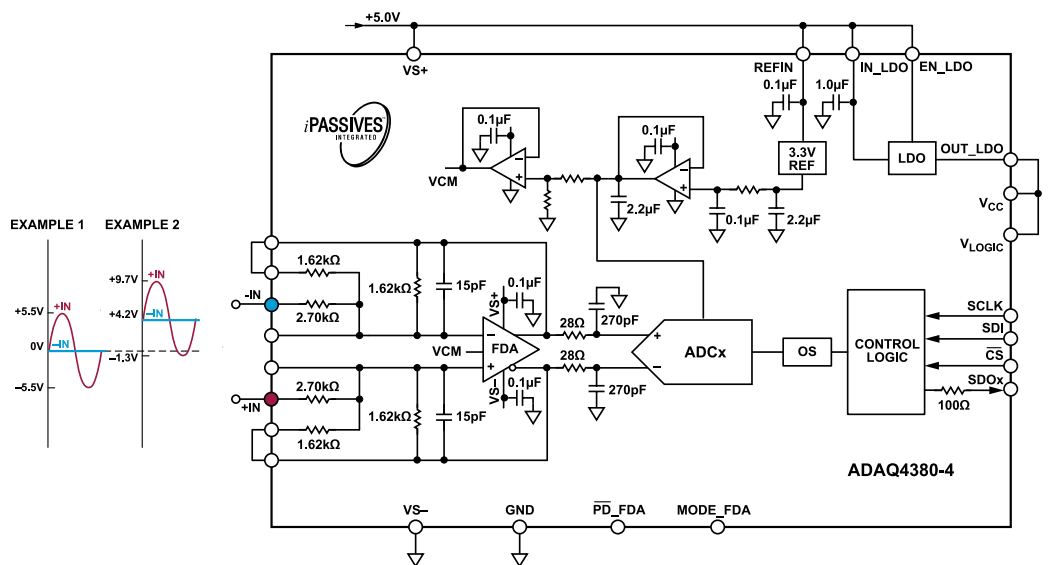
Figure 27. Single-Ended Input Configuration with Gain = 0.6, \pm 5.5 V Input, V_S = 5 V
