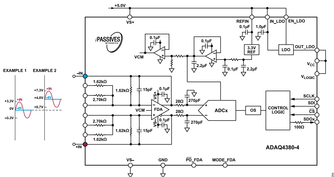
Figure 28. Single-Ended Input Configuration with Gain = 1.0, \pm 3.3 V Input, V_S = 5 V
