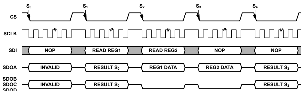
Figure 49. Register Read
