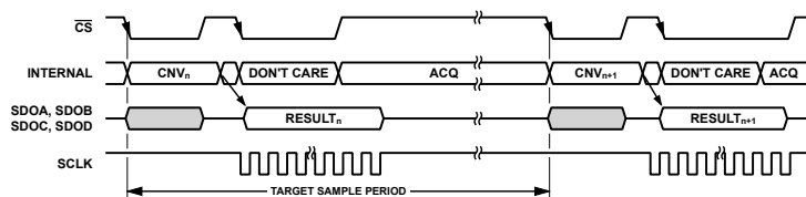
Figure 48. Low Throughput Low Latency
