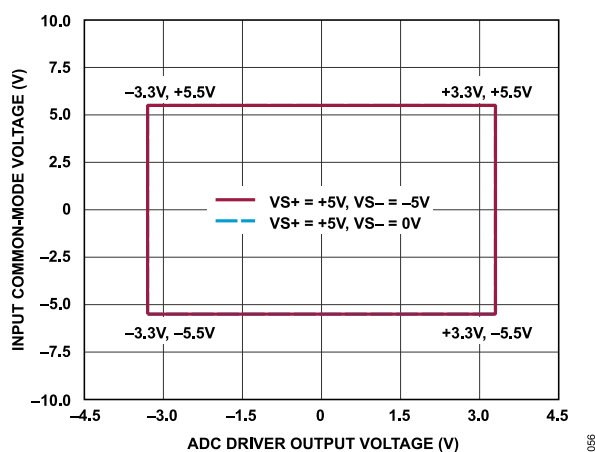
Figure 30. Input Common-Mode Voltage vs. ADC Driver Output, Gain = 0.3, \pm 11 V Differential Input
