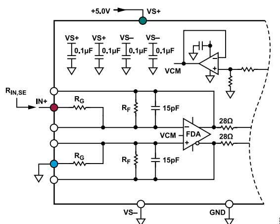
Figure 33. ADAQ4370-4 Configured at Single-Ended Inputs
