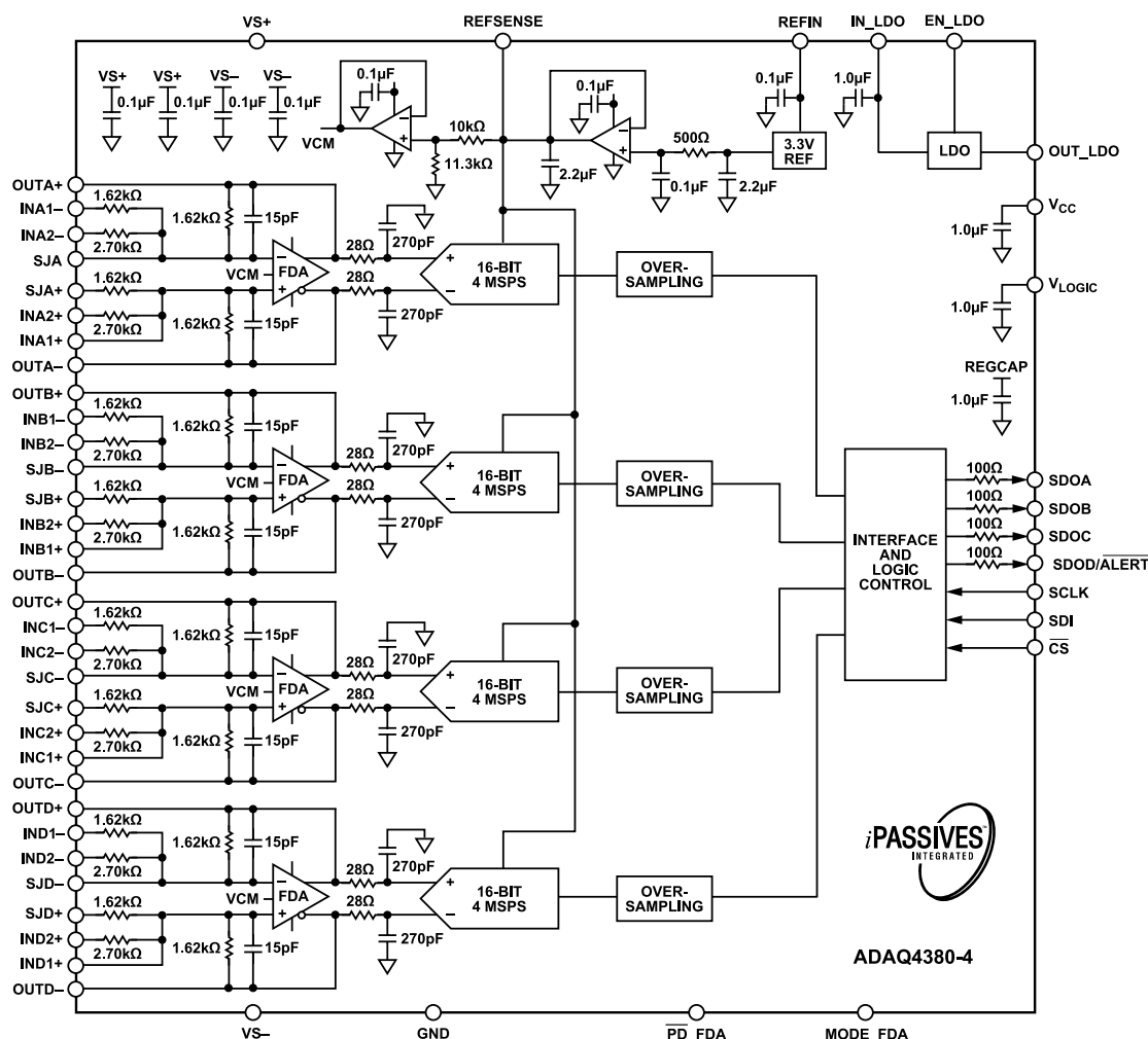
Figure 20. ADAQ4370-4 μModule Simplified Block Diagram
