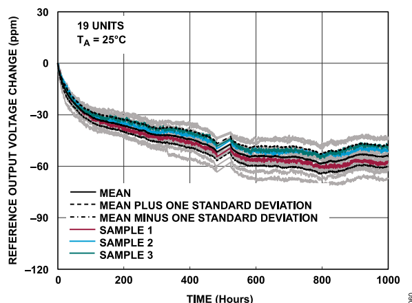
Figure 34. ADAQ4370-4 Internal Reference Long-Term Drift
