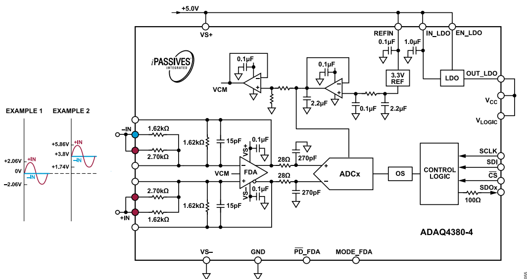
Figure 29. Single-Ended Input Configuration with Gain = 1.6, \pm 2.06 V Input, V_S = 5 V
