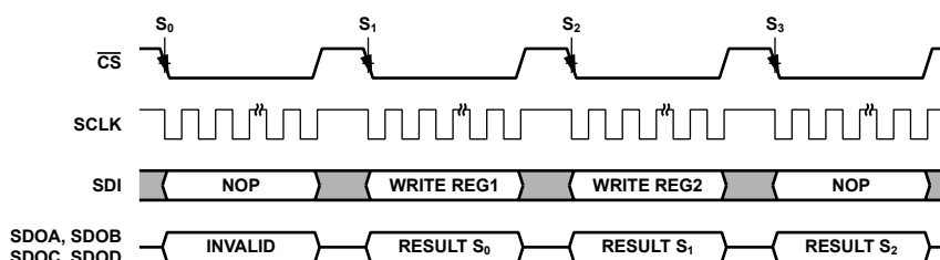
Figure 50. Register Write
