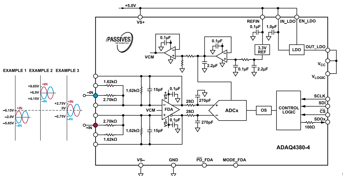
Figure 23. Fully Differential Input Configuration with Gain = 0.6, \pm 5.5 V Input, V_S = 5 V
