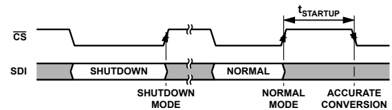
Figure 42. Shutdown Mode Operation
