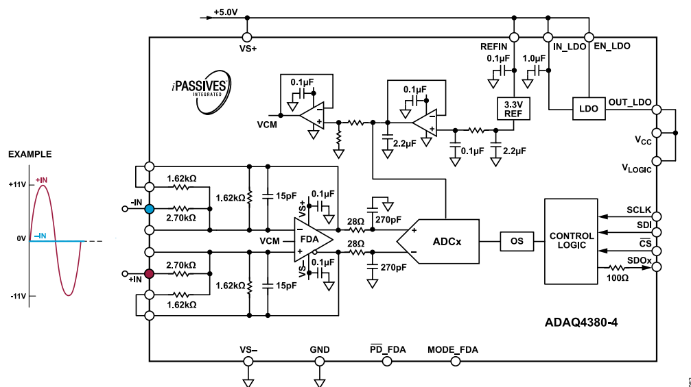
Figure 26. Single-Ended Input Configuration with Gain = 0.3, \pm 11 V Input, V_S = 5 V
