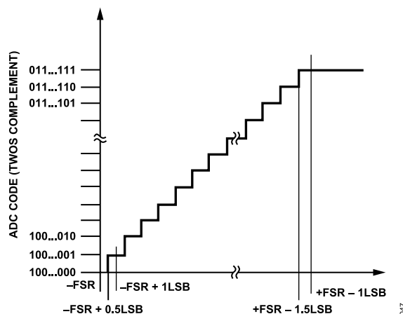
Figure 21. ADC Ideal Transfer Function (Full-Scale Range (FSR))
