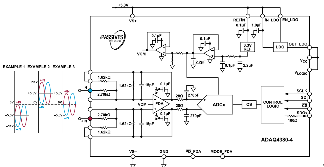
Figure 22. Fully Differential Input Configuration with Gain = 0.3, \pm 11 V Input, V_S = 5 V
