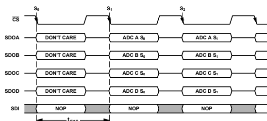
Figure 45. Read Conversion Results, 4-Wire Mode
