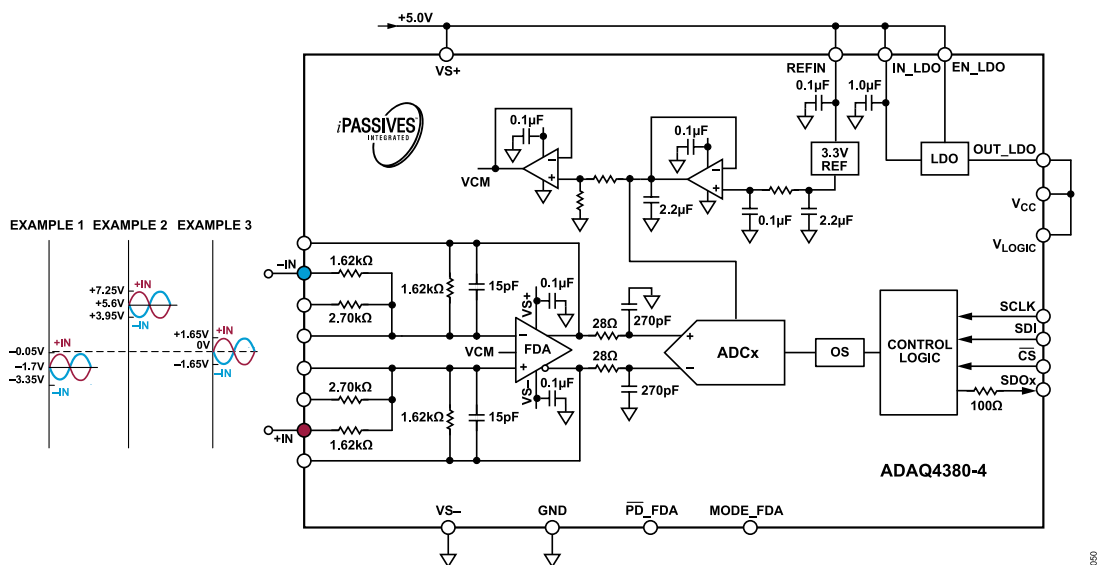
Figure 24. Fully Differential Input Configuration with Gain = 1.0, \pm 3.3\text{ V} Input, V_S = 5\text{ V}
