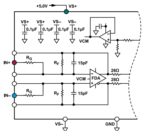
Figure 32. ADAQ4370-4 Configured at Fully Differential Inputs
