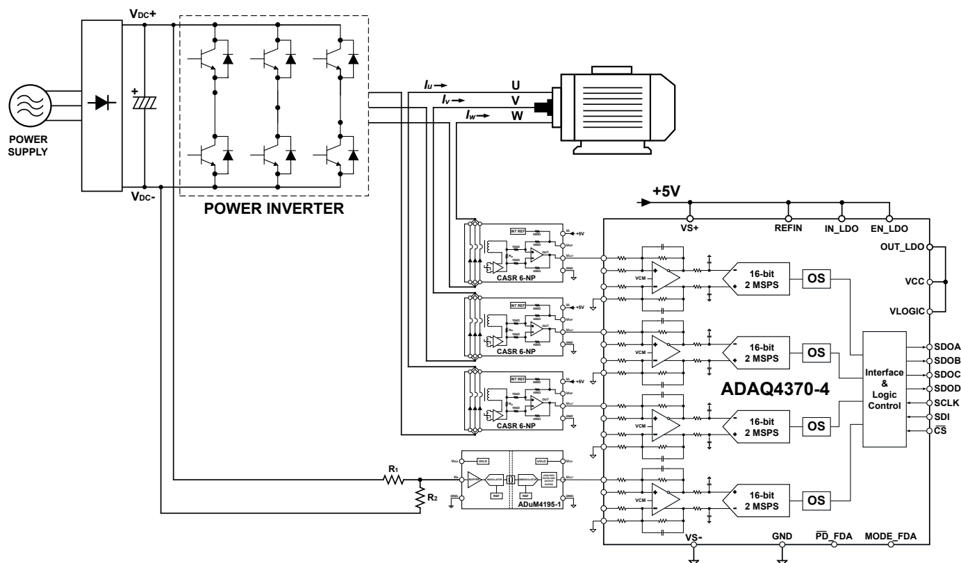
Figure 1. Precision Current and Voltage Sensing for Servo Motors Control using ADAQ4370-4
