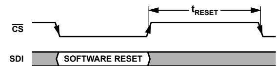
Figure 43. Software Reset Operation
