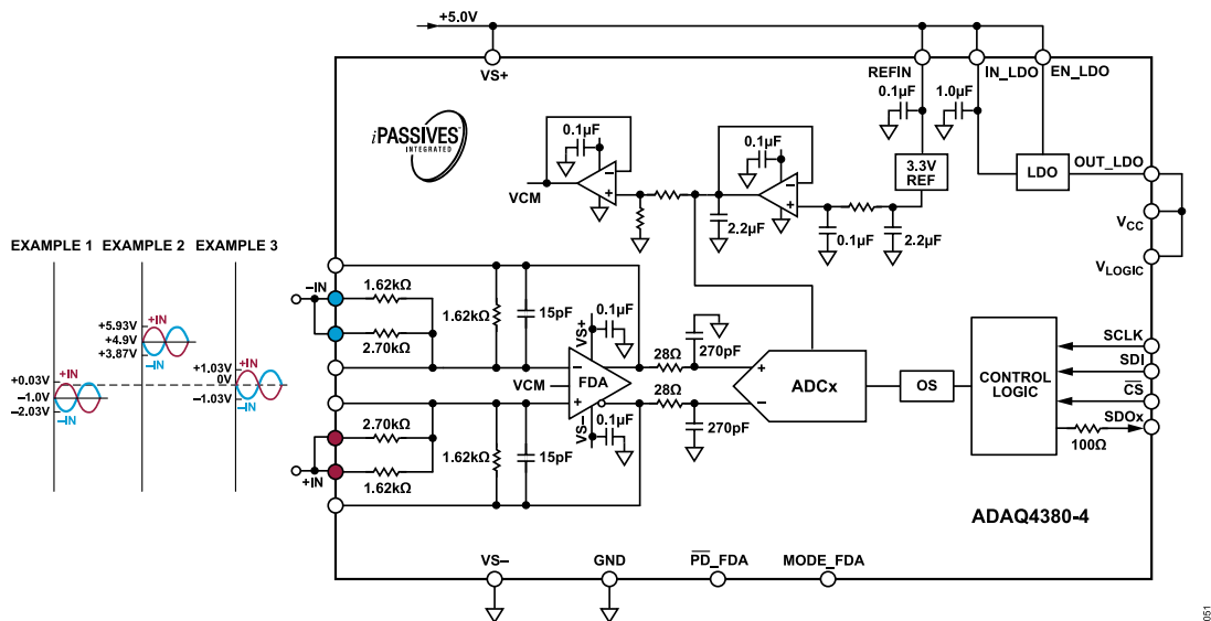
Figure 25. Fully Differential Input Configuration with Gain = 1.6, \pm 2.06\text{ V} Input, V_S = 5\text{ V}
