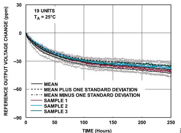
Figure 35. ADAQ4370-4 Internal Reference Early Life Drift
