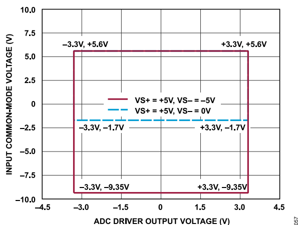
Figure 31. Input Common-Mode Voltage vs. ADC Driver Output, Gain = 1.0, \pm 3.3 V Differential Input
