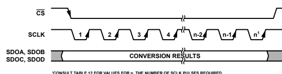
Figure 44. Reading Conversion Results
