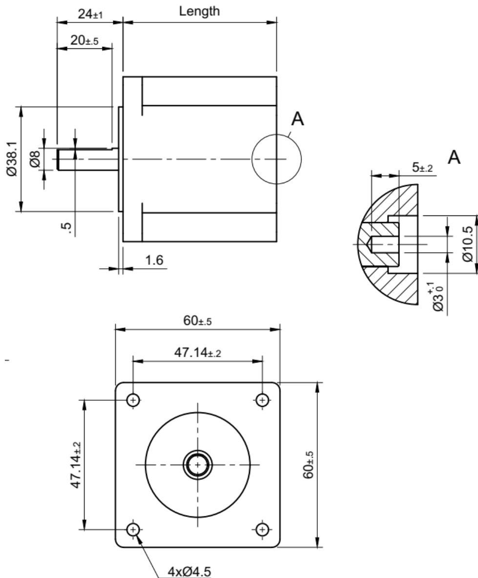
Figure 3.1: Dimensions (all values in mm)
