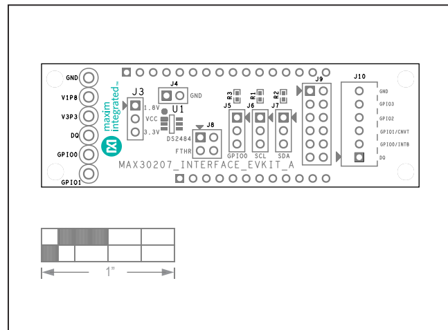
MAX30207EV Interface — Silk Top
