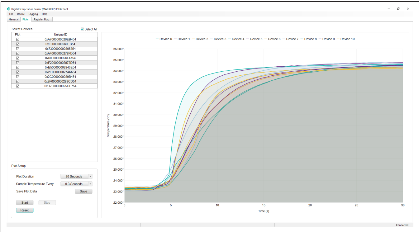
Figure 5. Plot Tab
