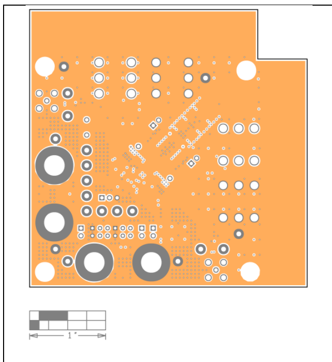
MAX20808 EV Kit PCB Layout—Layer 5
