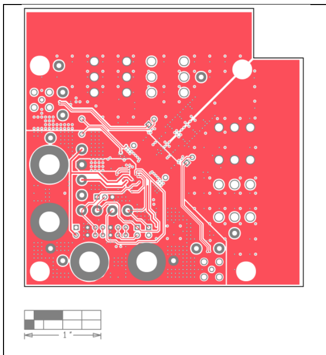
MAX20808 EV Kit PCB Layout—Layer 4
