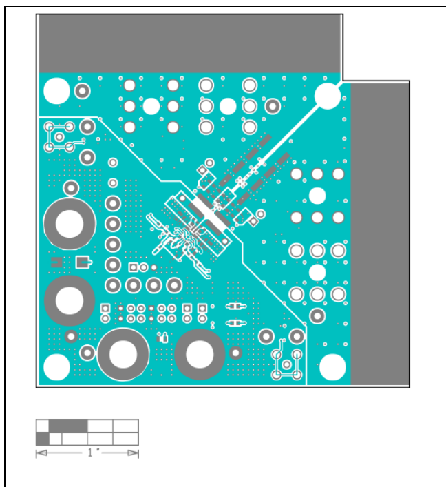
MAX20808 EV Kit PCB Layout—Top
