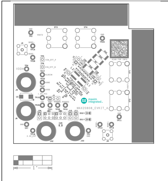
MAX20808 EV Kit Component Placement Guide—Top Silkscreen
