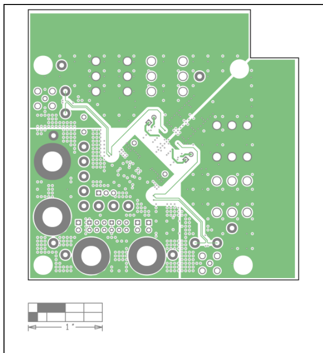
MAX20808 EV Kit PCB Layout—Layer 3
