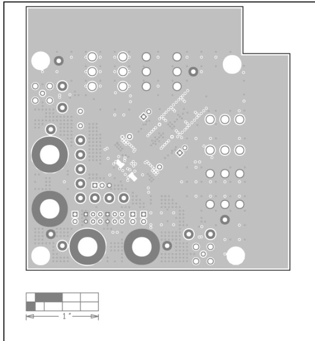
MAX20808 EV Kit PCB Layout—Layer 2
