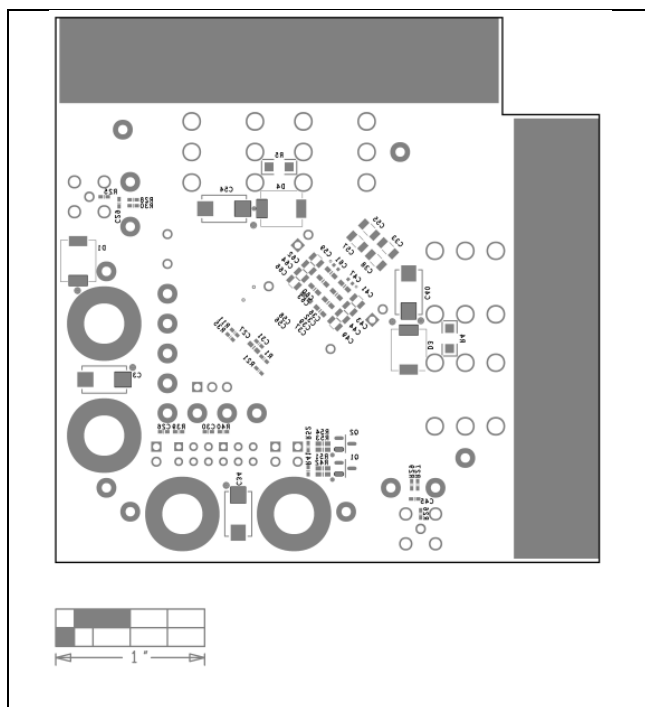
MAX20808 EV Kit Component Placement Guide—Bottom Silkscreen
