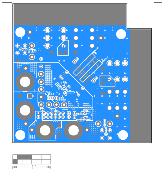
MAX20808 EV Kit PCB Layout—Bottom
