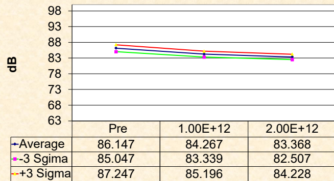
AVO RI=10k Side C
