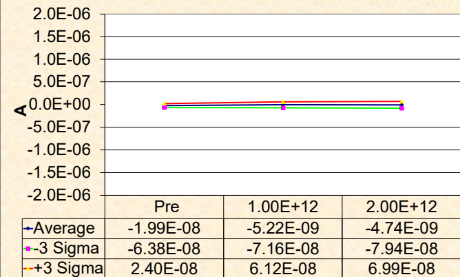
-Ibias Vcm=0V Side A
