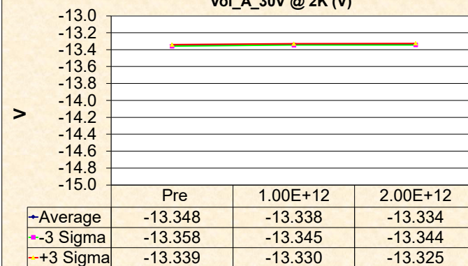
Vol_A_30V @ 2K (V)
