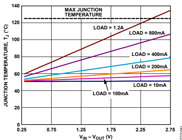
Figure 45. 1000 mm² of PCB Copper, T_B = 50^\circ\text{C} , LFCSP
