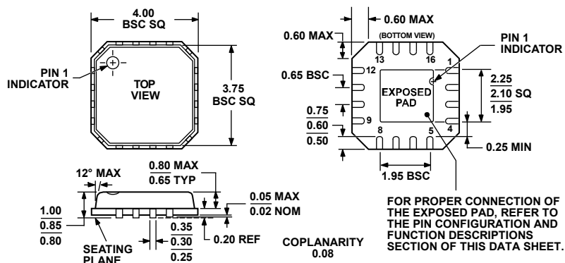
Figure 49. 16-Lead Lead Frame Chip Scale Package [LFCSP_VQ] 4 mm x 4 mm Body, Very Thin Quad (CP-16-4) Dimensions shown in millimeters
