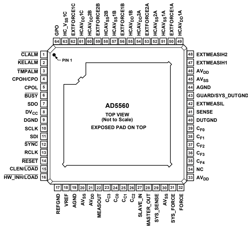
Figure 6. Pin Configuration
