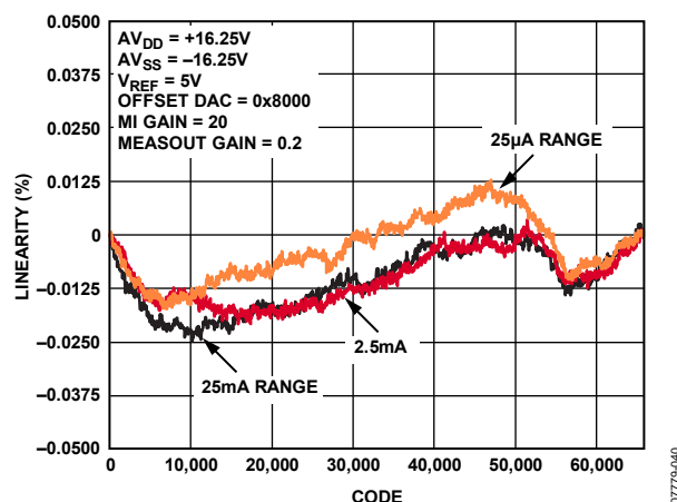
Figure 16. Measure Current Linearity vs. I_{\text{RANGE}} (MEASOUT Gain = 0.2, MI Gain = 20)
