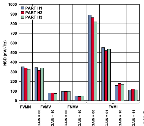
Figure 46. NSD vs. Amplifier Stage and Gain Setting at 1 kHz
