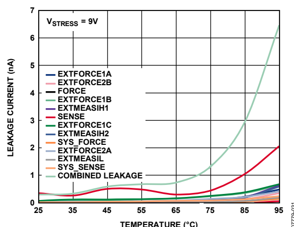
Figure 18. Leakage Current vs. Temperature (Force and Combined Leakage), V_{\text{STRESS}} = 9V
