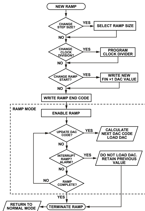
Figure 56. Flow Chart for Ramp Function
