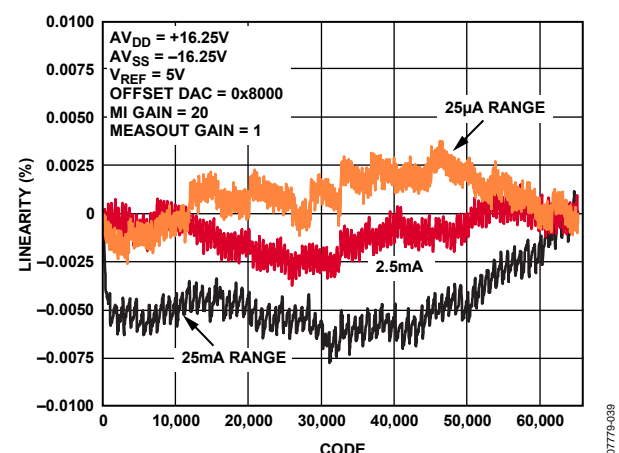
Figure 15. Measure Current Linearity vs. I_{\text{RANGE}} (MEASOUT Gain = 1, MI Gain = 20)
