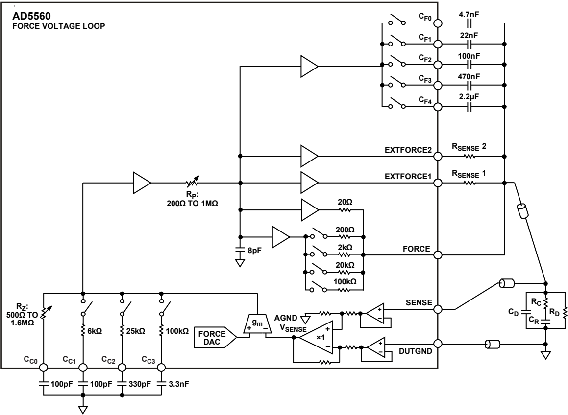
Figure 55. Block Diagram of Force Amplifier Loop
