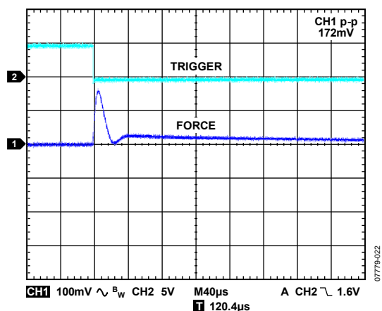
Figure 36. Safe Mode 80% to 10% I_{LOAD} Change, EXTFORCE2 Range, 10 µF Load
