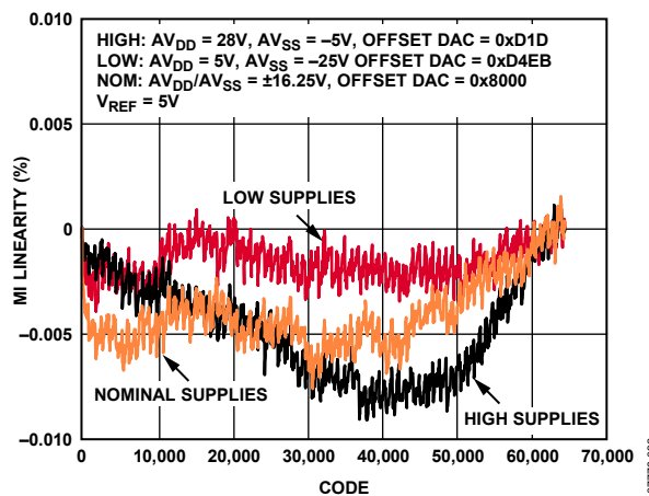
Figure 12. Measure Current Linearity vs. Code (MEASOUT Gain = 1, MI Gain = 10)
