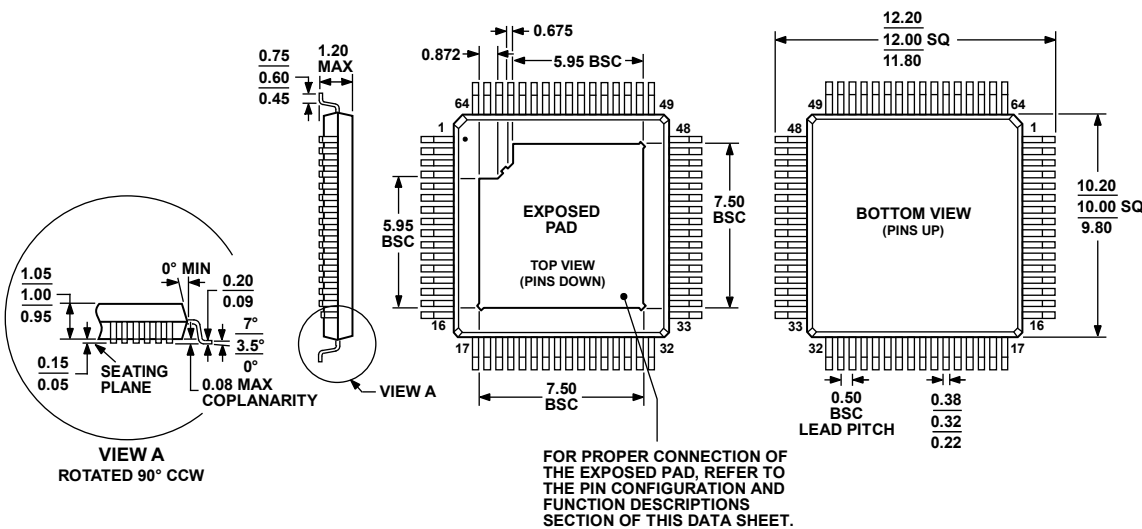
COMPLIANT TO JEDEC STANDARDS MS-026-ACD-HU Figure 59. 64-Lead Thin Quad Flat Package, Exposed Pad [TQFP_EP] (SV-64-3) Dimensions shown in millimeters
