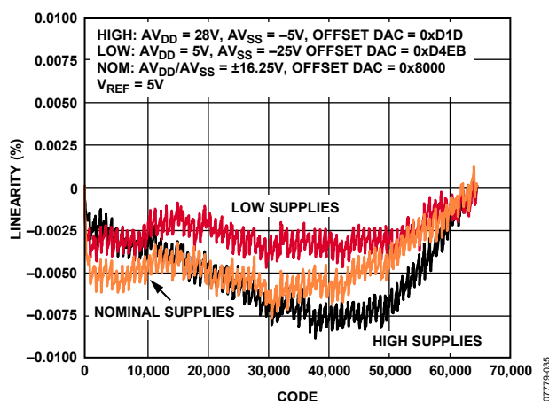
Figure 11. Measure Current Linearity vs. Code (MEASOUT Gain = 1, MI Gain = 20, TJ = 25°C)
