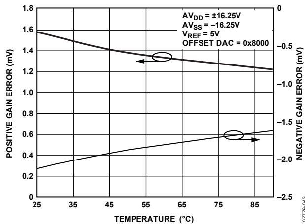
Figure 23. FV Gain Error vs. Temperature
