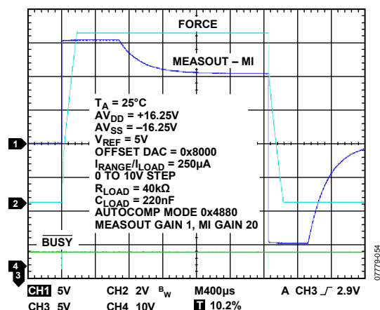
Figure 39. Transient Response FVMI Mode, \pm 250 \mu A Range, Autocompensation Mode
