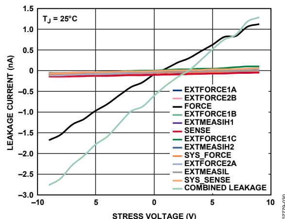
Figure 17. Leakage Current vs. Stress Voltage (Force and Combined Leakage)
