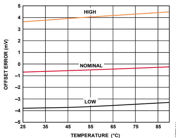
Figure 28. MV Offset Error vs. Temperature, MEASOUT Gain = 0.2
