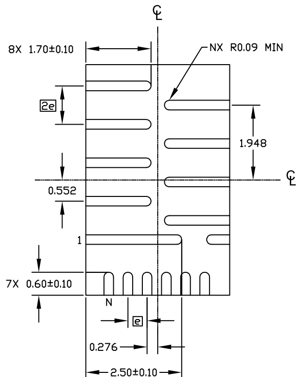
BOTTOM VIEW
