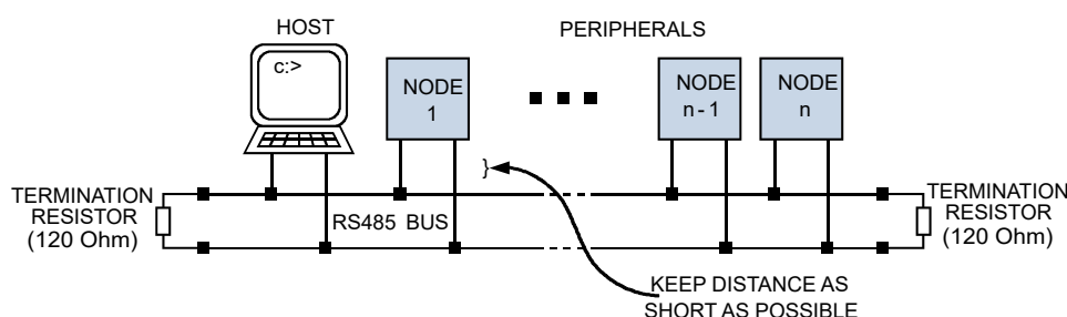
Figure 17: RS485 Bus Structure with Termination Resistors
