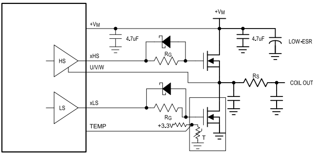
Figure 15: Thermistor Implementation
