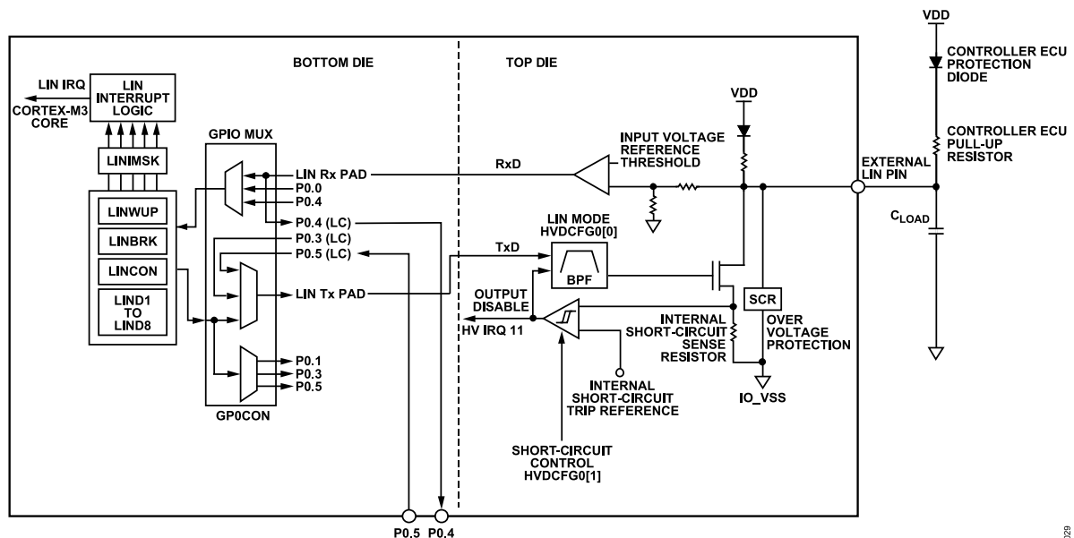
Figure 29. LIN Block Diagram
