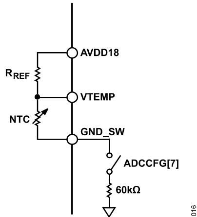
Figure 16. Internal Ground Switch Configuration
