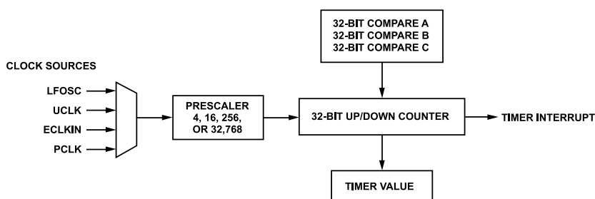
Figure 20. General-Purpose Timers Block Diagram
