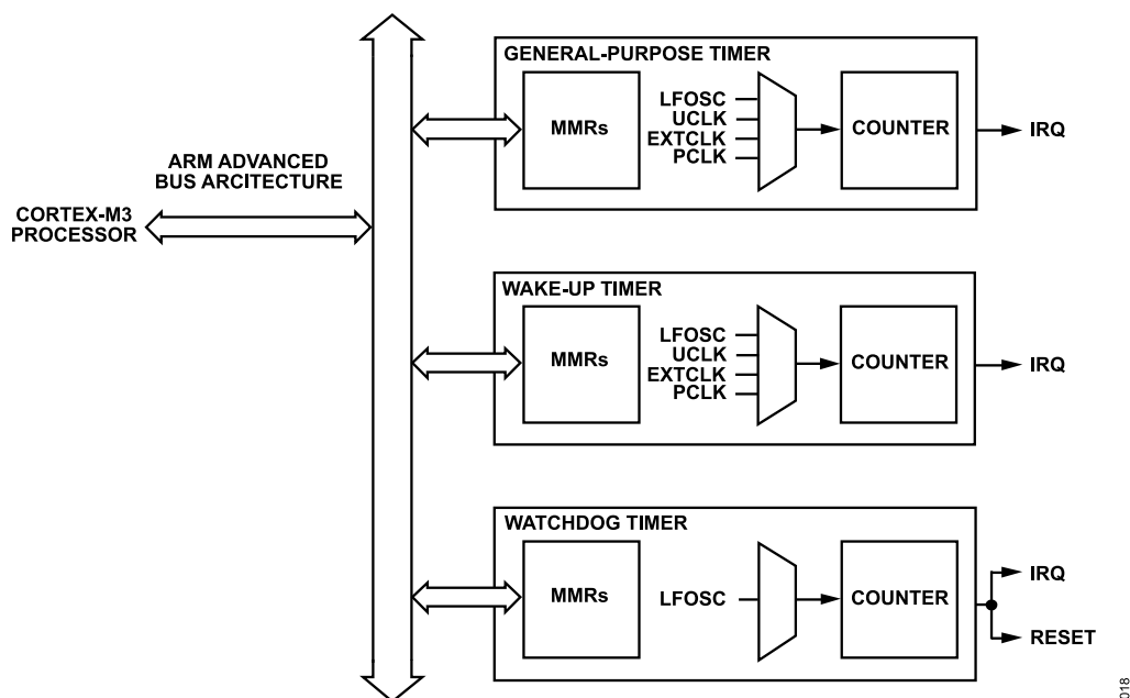
Figure 18. Timer Synchronization Block Diagram
