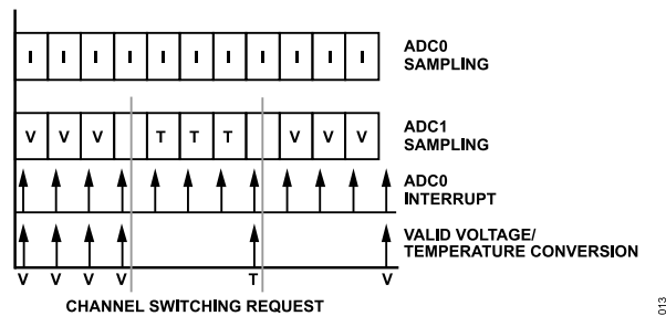
Figure 13. Default Temperature Mode, Chop Off
