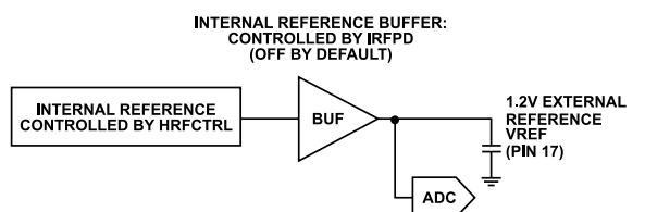
Figure 15. ADC Reference Configuration
