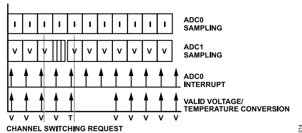
Figure 14. Fast Temperature Mode, Chop Off (ADCFLT = 0x07)
