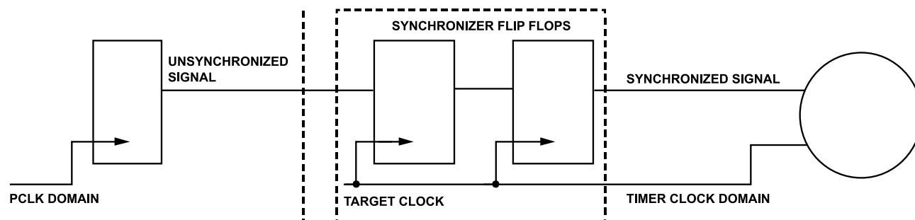
Figure 19. Synchronizer for Signals Crossing Clock Domains
