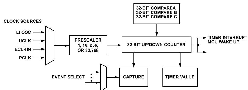
Figure 21. Wake-Up Timer Block Diagram
