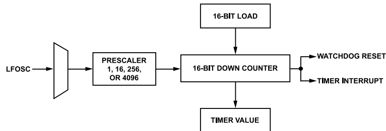
Figure 22. Watchdog Timer Block Diagram
