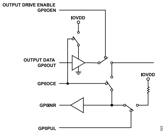
Figure 23. GPIO Block Diagram
