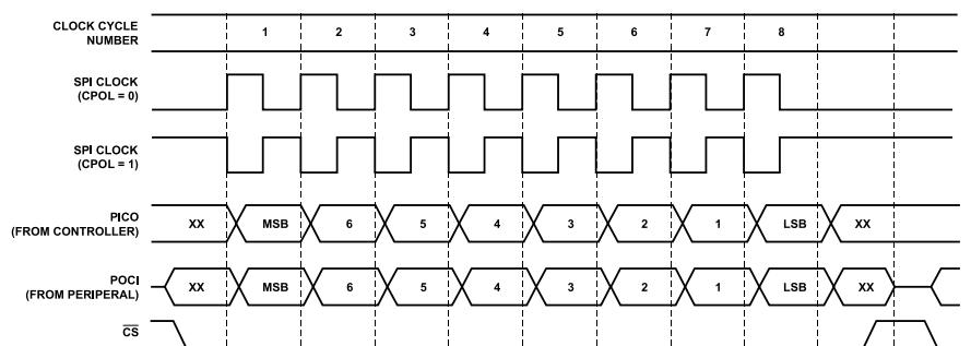
Figure 26. SPI Transfer Protocol, CPHA = 1
