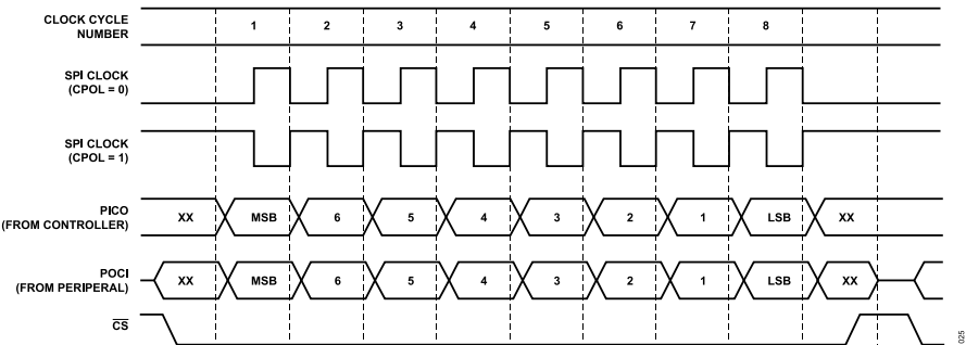
Figure 25. SPI Transfer Protocol, CPHA = 0
