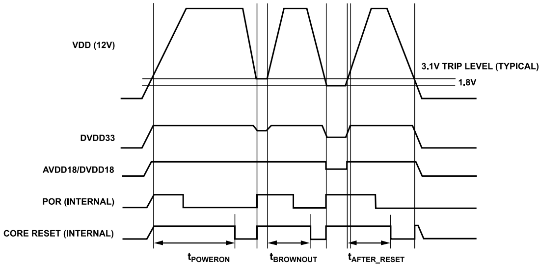
Figure 1. Power Supply Diagram
