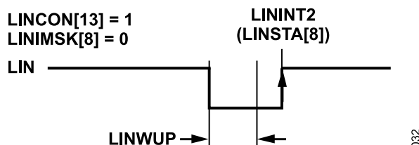
Figure 32. Wake-Up Interrupt
