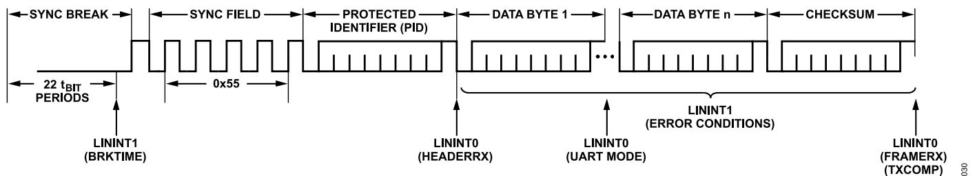
Figure 30. LIN Interrupts
