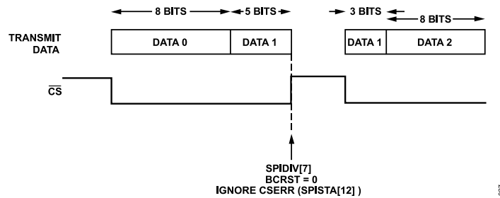
Figure 27. Serial Peripheral Interface, Erroneous Deassertion of Chip Select Diagram
