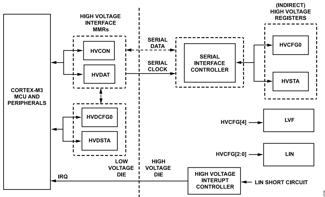
Figure 28. High Voltage Interface, Top Level Block Diagram
