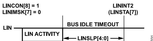
Figure 31. Sleep Interrupt
