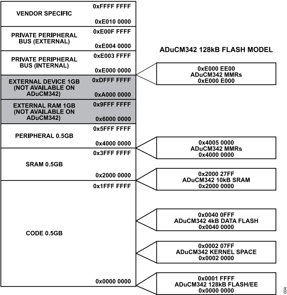
Figure 4. Memory Map Diagram
