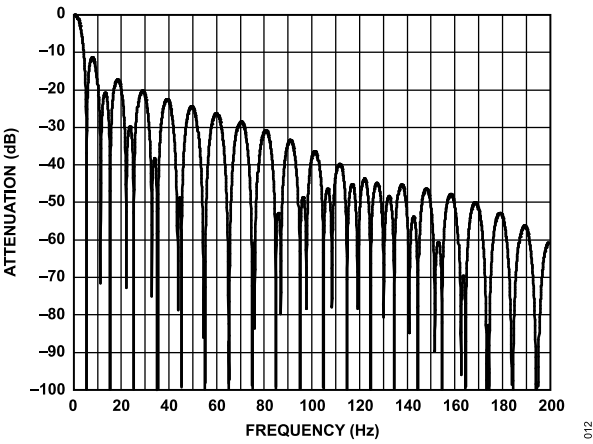
Figure 12. Typical Digital Filter Response at f_{\text{ADC}} = 10 \text{ Hz} ( \text{ADCFLT} = 0x961F )
