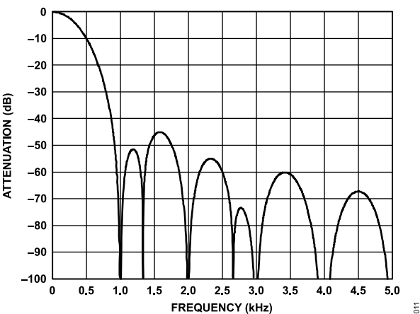
Figure 11. Modified Sinc3 Digital Filter Response at f_{\text{ADC}} = 1.0 \text{ kHz} ( \text{ADCFLT} = 0x0087 )
