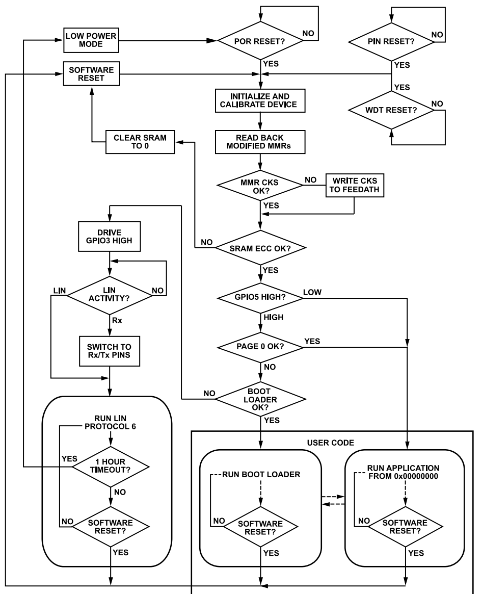
Figure 3. Kernel Flowchart
