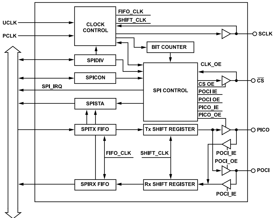
Figure 24. SPI Block Diagram
