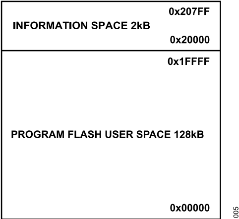
Figure 5. Program Flash Memory Map
