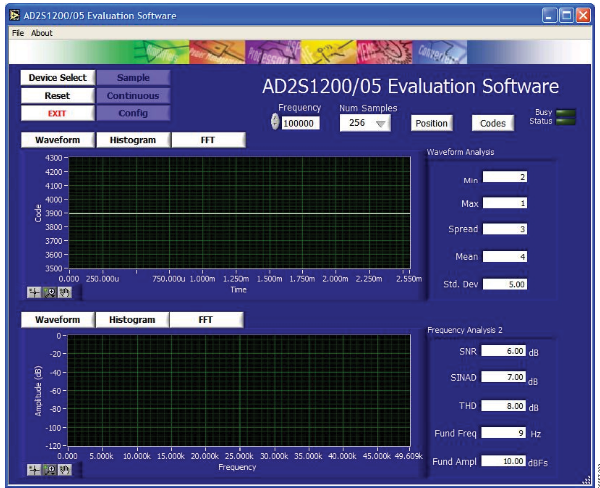
Figure 3. AD2S1200/05 Evaluation Software, Main Window
