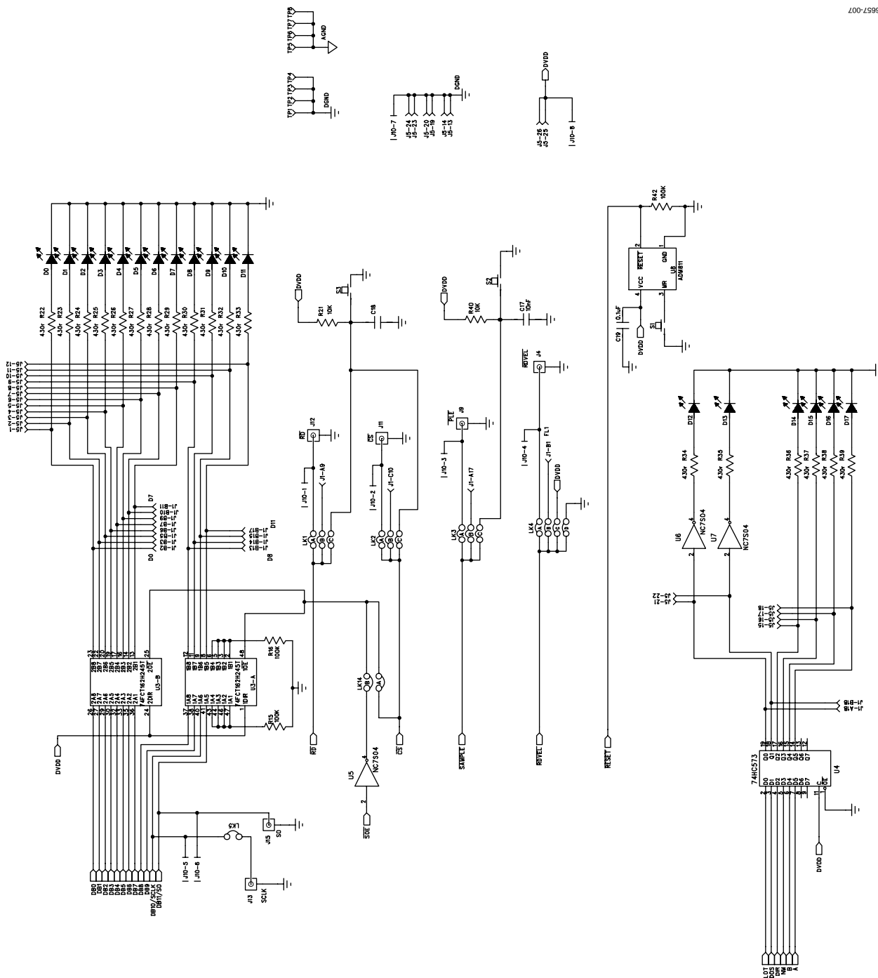
Figure 7. EVAL-AD2S1200/AD2S1205 Schematic—Page 3
