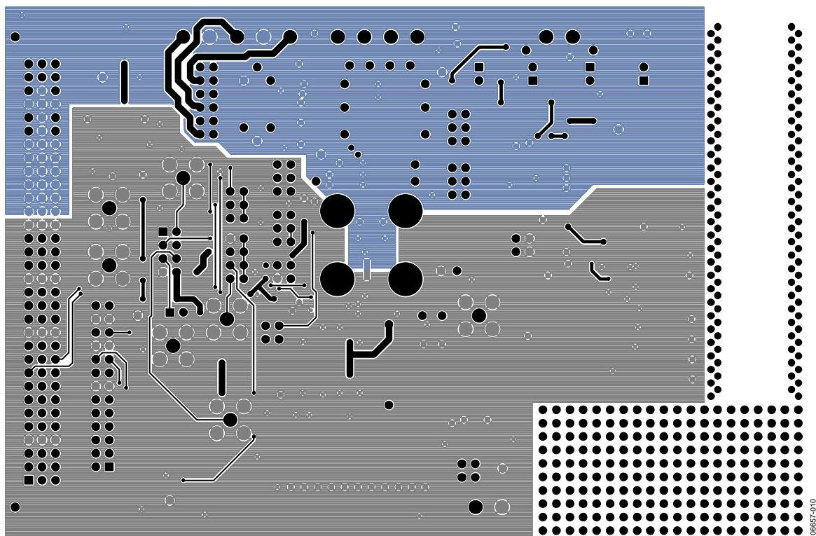
Figure 10. Solder Side
