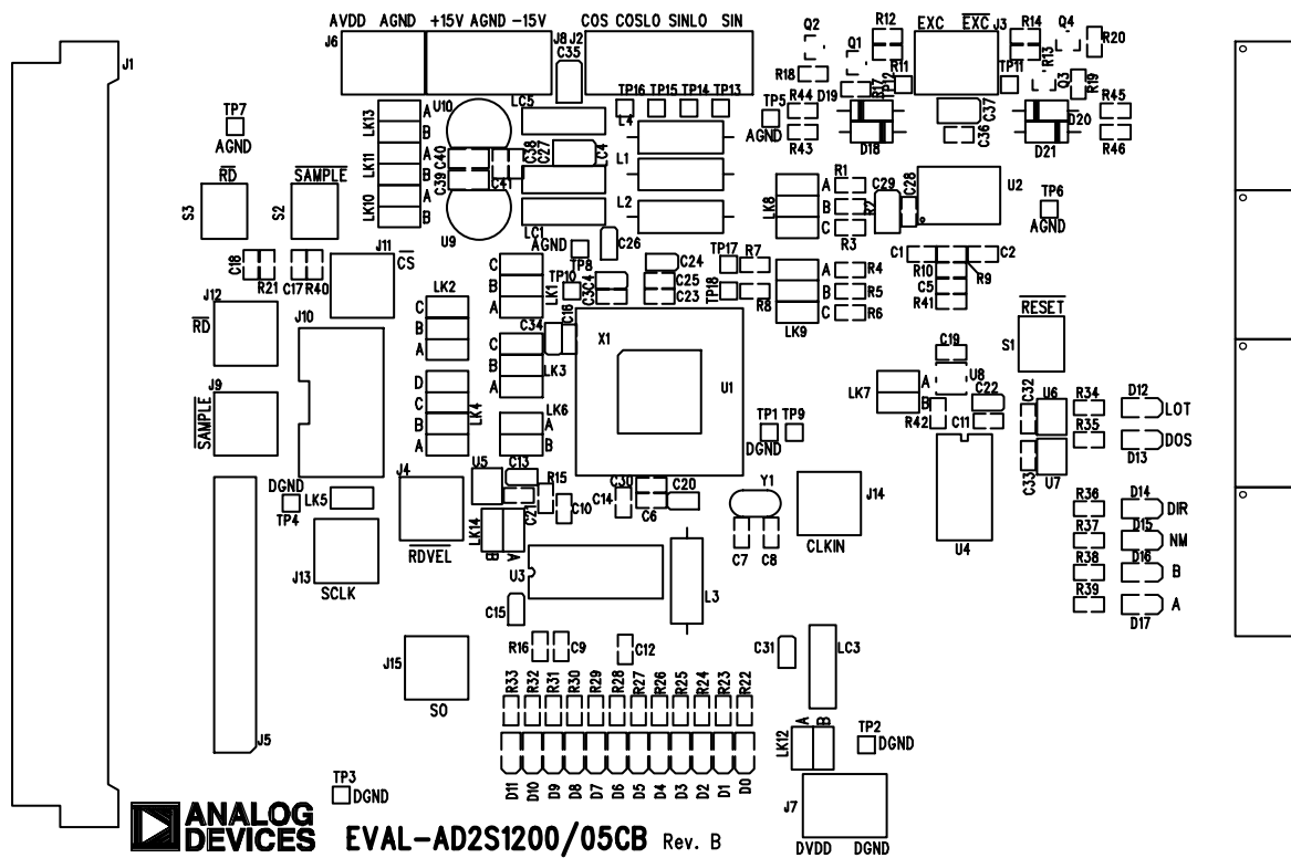
Figure 8. Silkscreen Image
