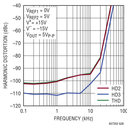
谐波失真与频率的关系, G = 0.25 , R_L = 2\text{k}\Omega
