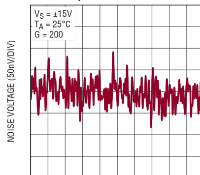
0.1Hz至10Hz噪声电压, G = 200, RTI
