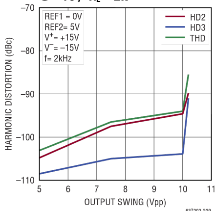
谐波失真与输出摆幅的关系, G = 10 , R_L = 2\text{k}\Omega
