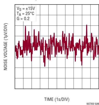
0.1Hz至10Hz噪声电压, G = 0.2 , RTI
