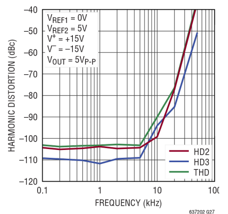
谐波失真与频率的关系, G = 1 , R_L = 2\text{k}\Omega
