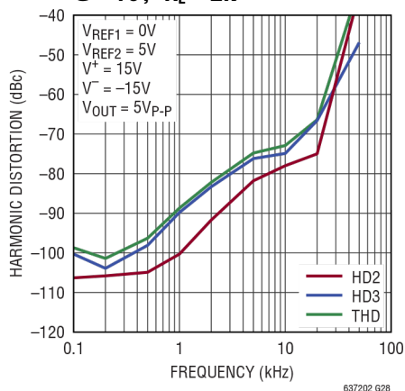
谐波失真与频率的关系, G = 10 , R_L = 2\text{k}\Omega
