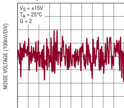
0.1Hz至10Hz噪声电压, G = 2, RTI
