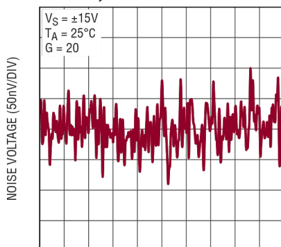
0.1Hz至10Hz噪声电压, G = 20, RTI
