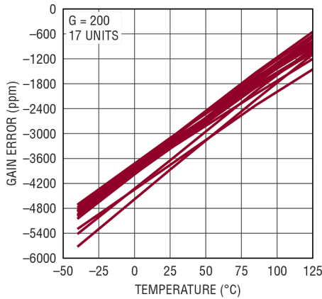
增益漂移( G = 200 )
